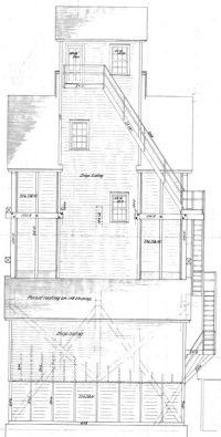
Rear Elevation
